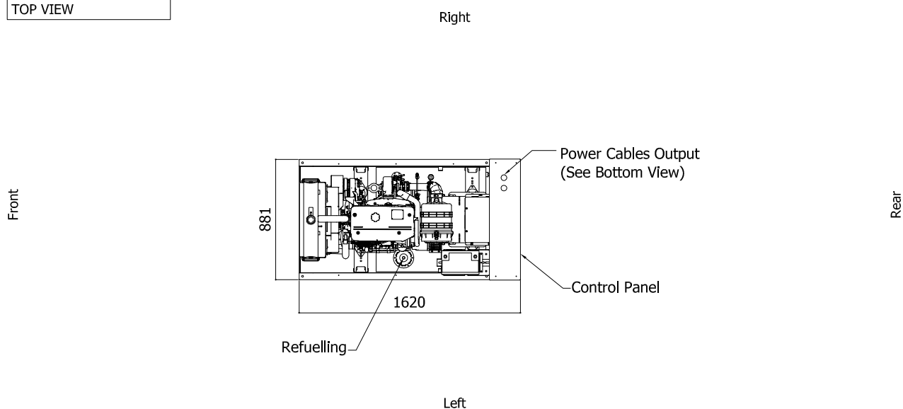
TOP VIEW
